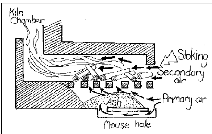
Fig.2-49: Function of a wood firebox. The height of ash pit should equal the height above the gate.
