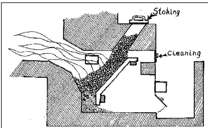
Fig.2-63: Stoking of a semi-gas producer.
