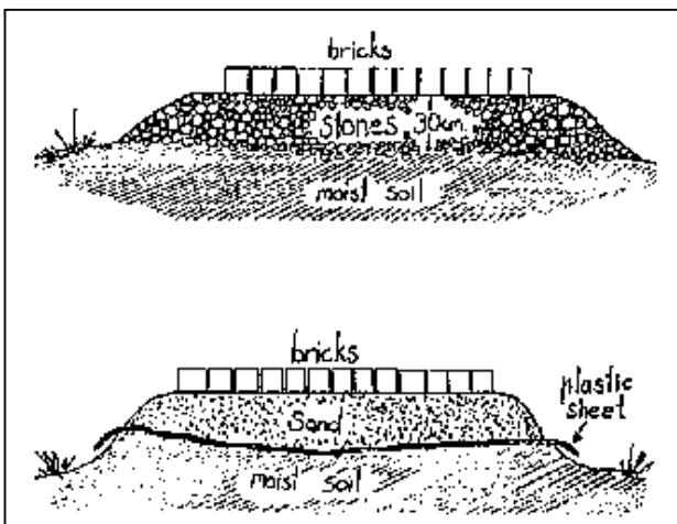
Fig.2-78: A layer of stone pebbles seals off the moisture
