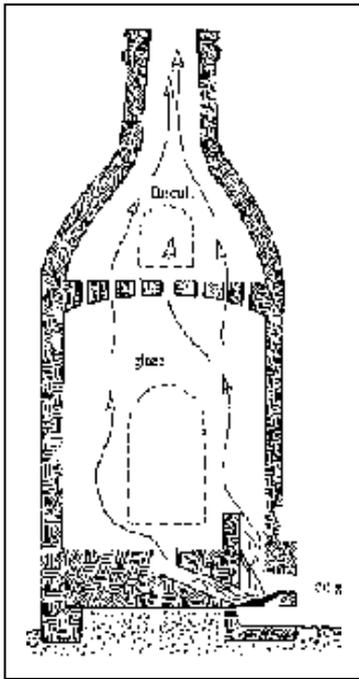
Fig.2-12: Bottle kiln with its innovations: chimney, firebricks and iron grates for burning coal.
