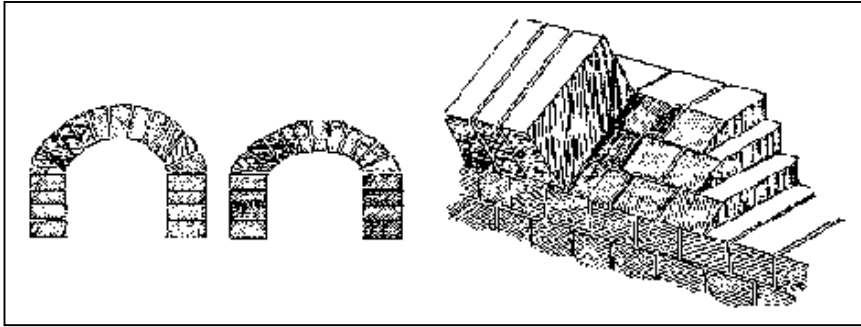
Fig.2-90: Firebox arch after construction, and later after firing shrinkage of the firebricks has taken place. The initial high rise saved the firebox arch from collapsing due to firing shrinkage; Fig.2-91: Skewbacks cut from square bricks
