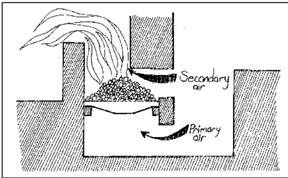
Fig.2-61: Coal firebox with flat grates.
