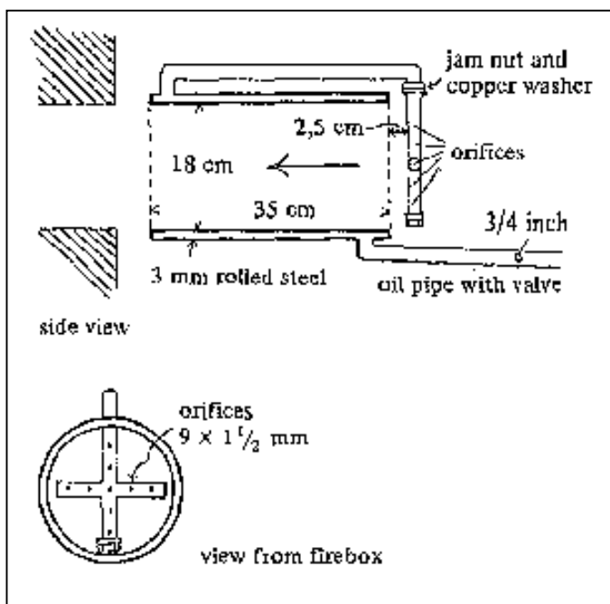
Fig.2-70: Large pressure burner.
