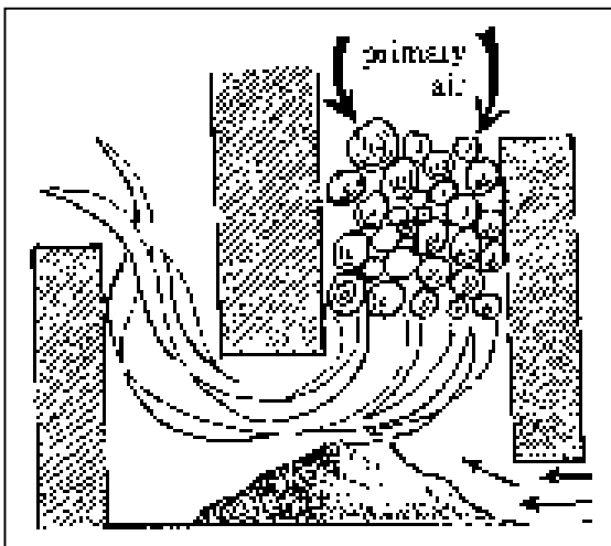
Fig.2-52: Hob firebox.
