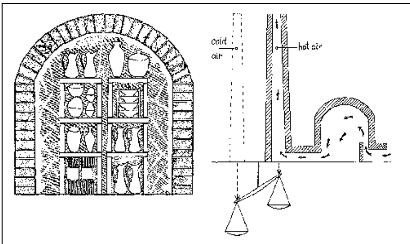
Fig.2-72: At red heat the kiln walls will radiate heat back to the kiln setting. Fig.2-73: The hot air the chimney weighs much less than cold air of the same volume. The balance illustrates this weight difference.
