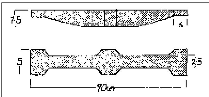
Fig.2-60: Typical grate bars for coal. The thickened parts adjust the open space between the bars.
