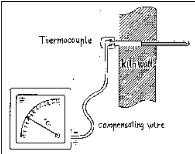
Fig.2-140: Pyrometer
