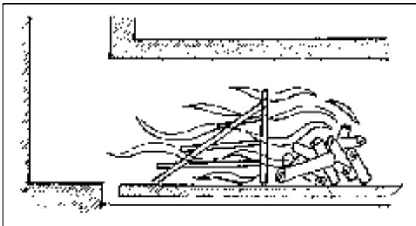
Fig.2-68: Preheating of burner plates
