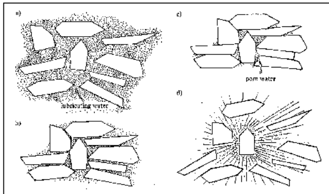
Fig.2-131: Clay shown in four stages. The clay crystals are made 100 000 times larger than their real size.
