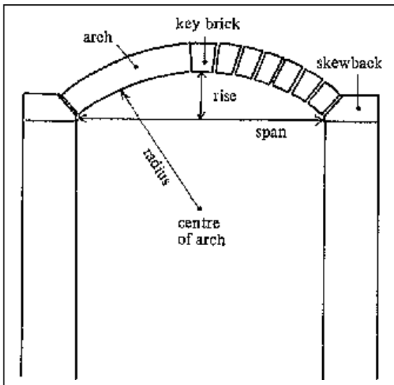
Fig.2-89: Arch.
