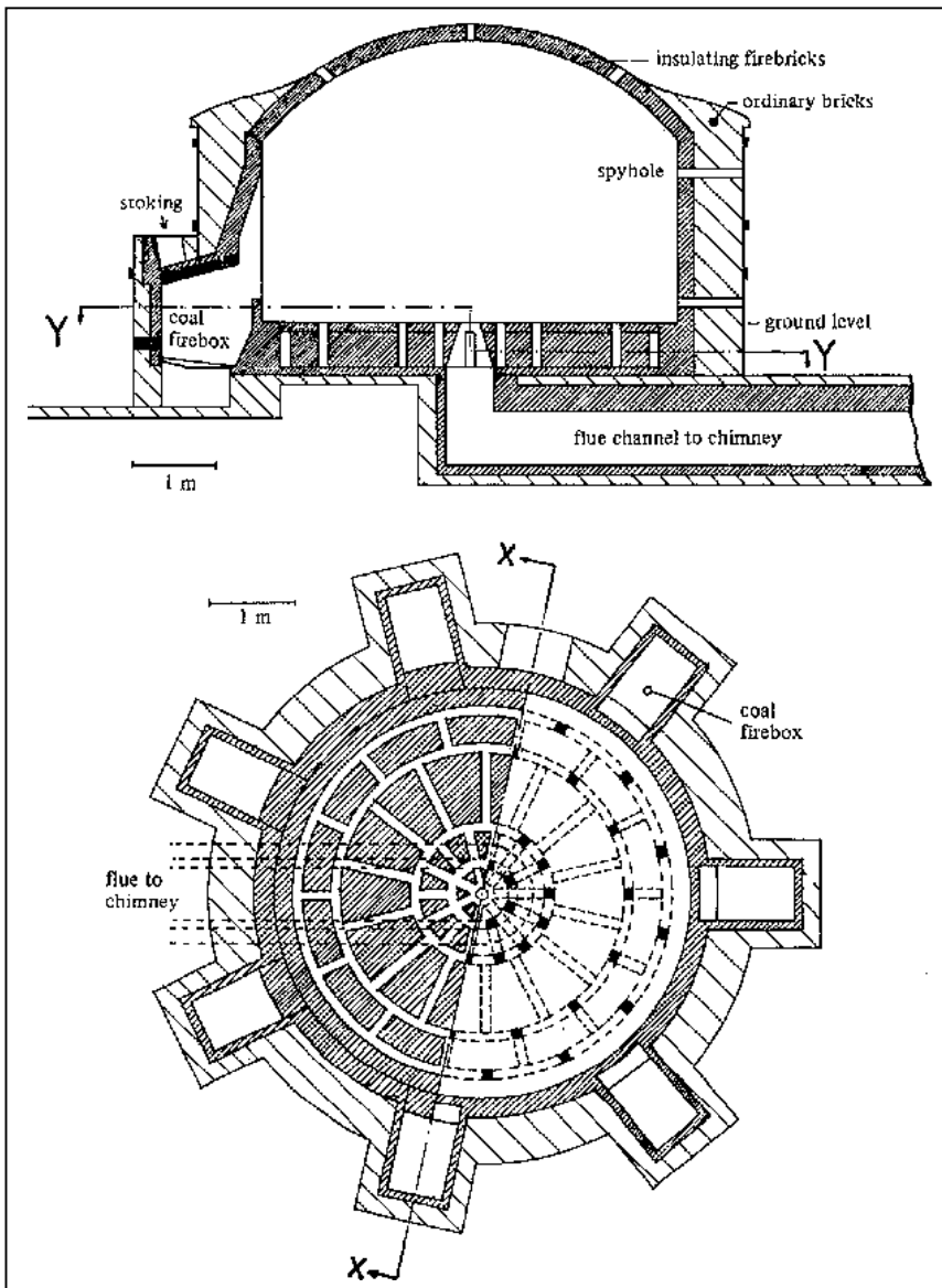
Fig.2-19: Khurja down-draught kiln a) side elevation, b) ground elevation showing flue holes and channels. The details for this kiln have been obtained from "Status Report on Ceramic Industry at Khurja", published by Central Glass and Ceramic Research Institute, Calcutta, India.
