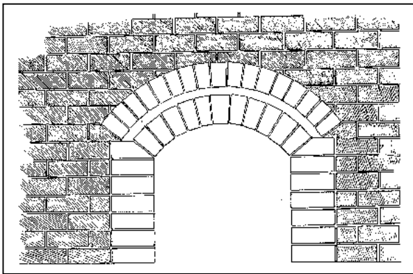
Fig.2-92: Relieving arch.
