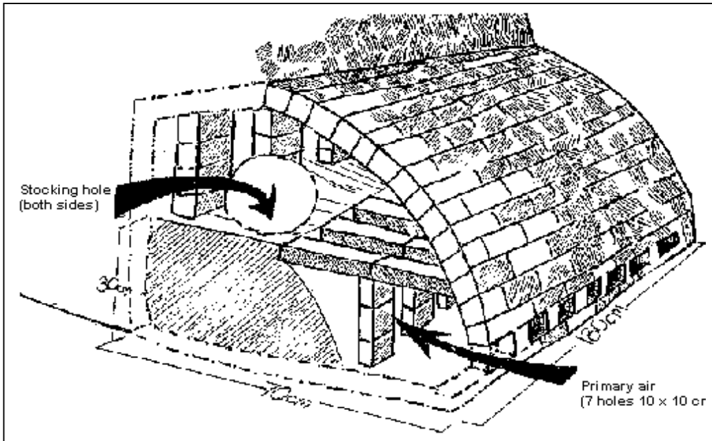
Fig.2-34: Champaknagar firebox.
