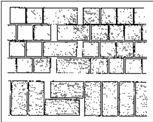
Fig.2-108: Expansion joints in a kiln wall. Side elevation. Fig.2-109: The same expansion joints as in fig. 2-108 seen from the top of the wall.
