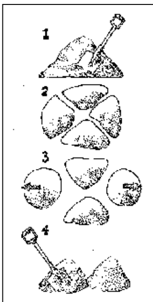
Fig.1-47: The method of quartering: 1.The sample is mixed well. 2.It is then divided into four portions. 3.Two portions are removed. 4.The remaining two portions are mixed well and another cycle of quartering can start.
