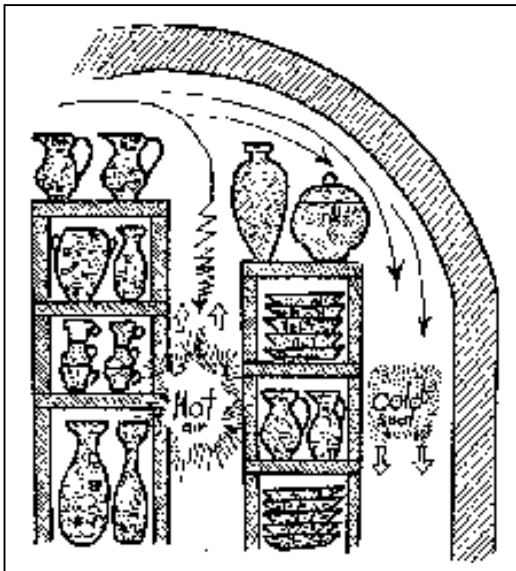
Fig. 2-17: The downward draught avoids the hot spots and seeks out the cold spots in the kiln setting.
