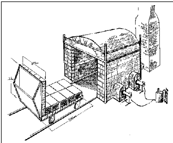
Fig.2-71: 2 m 3 down-draught shuttle kiln with four small pressure burners. Exit flue is in the bottom of the shuttle car.
