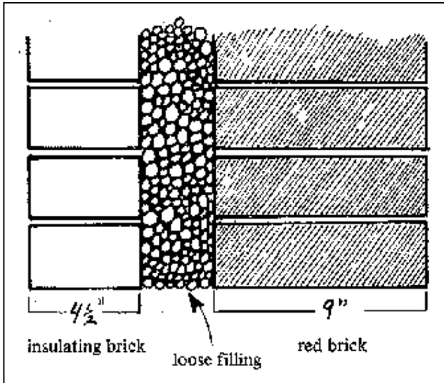
Fig.2-87: Cross-cut of a circular kiln wall.
