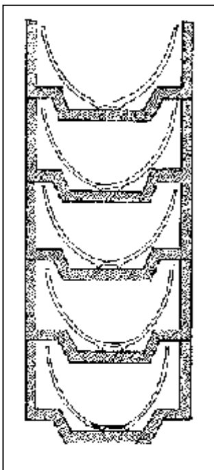
Fig. 1-16: Saggars shaped for dense setting of blows
