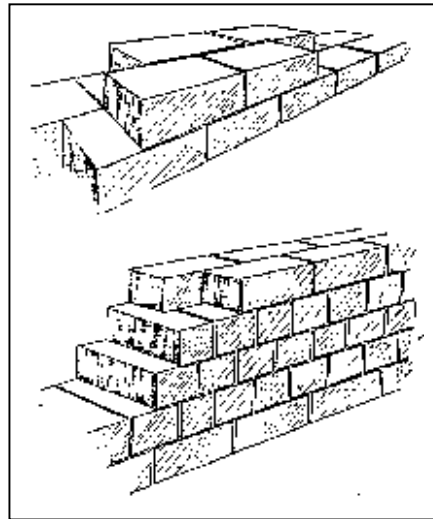
Fig.2-84: One stretcher course for each three header courses. Fig.2-85: Stretcher courses in a Chinese-type tube kiln.
