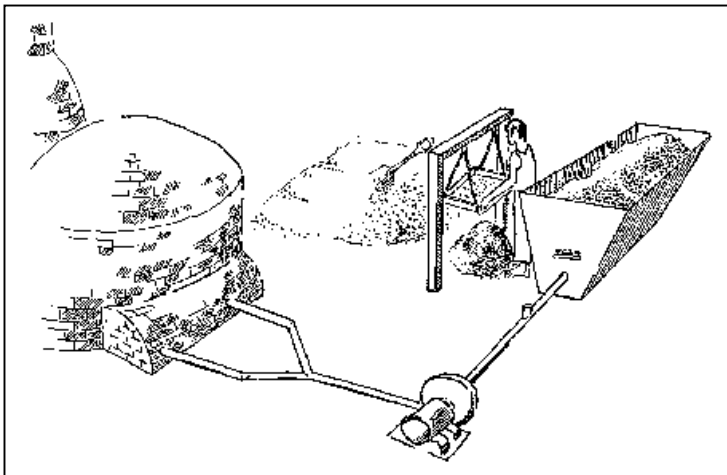
Fig.2-55: Sawdust injection system.
