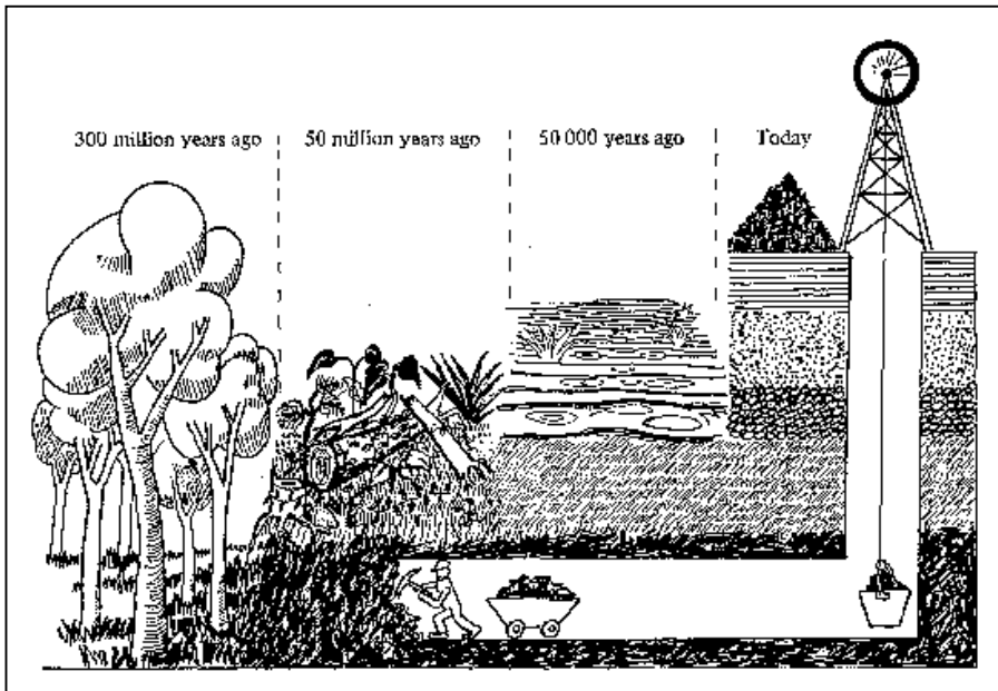
Fig.2-43: Peat, lignite and coal are created by forests growing in ancient times. The starting point for coal formation is peat and as this is compacted more and more it is converted into lignite and finally into coal. Peat found today may be only a few thousand years old whereas lignite may be 50 million years old and coal up to 300 million years.
