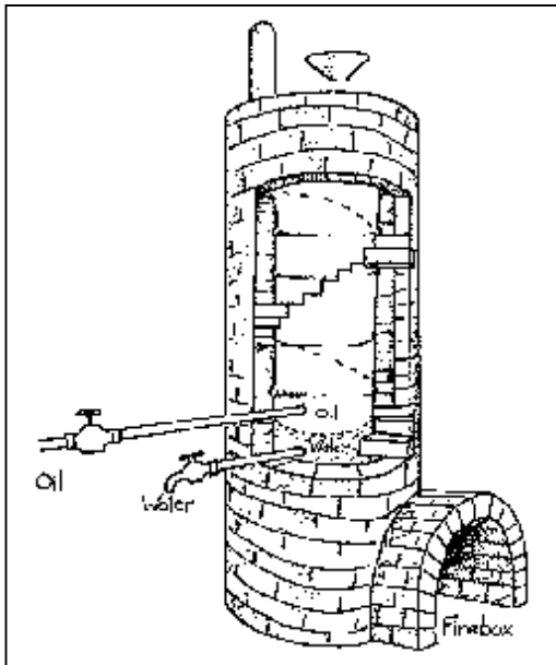
Fig.2-67: Oil tank for separation of water and heating of the fuel oil. In fig.2-35 a photograph of such an oil tank is shown
