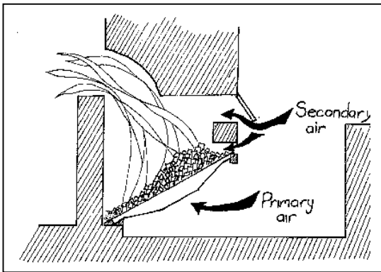
Fig.2-62: Coal firebox similar to the ones seen in fig.2-59. The firebox is within the outer wall of the kiln. Secondary air is regulated by opening of the stoking shutter and by placement of bricks just above the grate bars.
