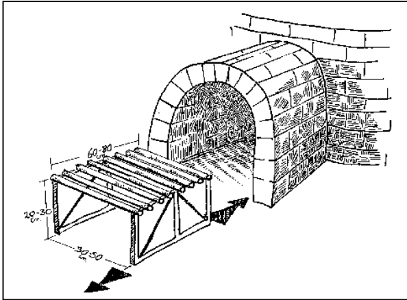
Fig.2-51: Iron grates will last longer if they can be removed after firing has been finished (F.Olsen "The Kiln Book" fastfire wood kiln).
