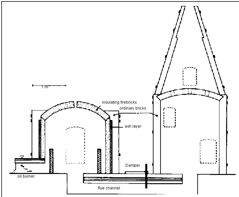
Fig.2-24: Two-chamber Bujora kiln, cross-section. The first chamber is provided with three fireboxes for oil firing but fireboxes for firewood or coal could be used as well.
