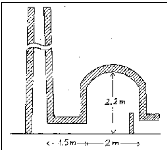
Fig.2-74: Kiln with downward pull of 2.2 m and horizontal pull of 3.5 m.
