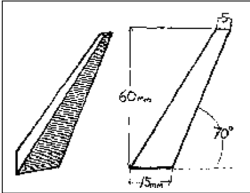
Fig.2-141: Shape and dimension of cones.
