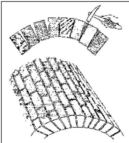
Fig.2-96: Square brick arch. Fig.2-97: Bonded arch
