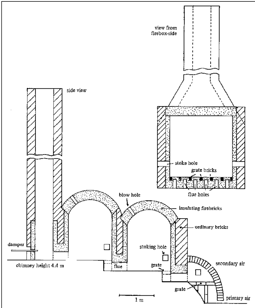
Fig.2-33: Two-chambered wood-fired kiln. Champaknagar, Banladesh.
