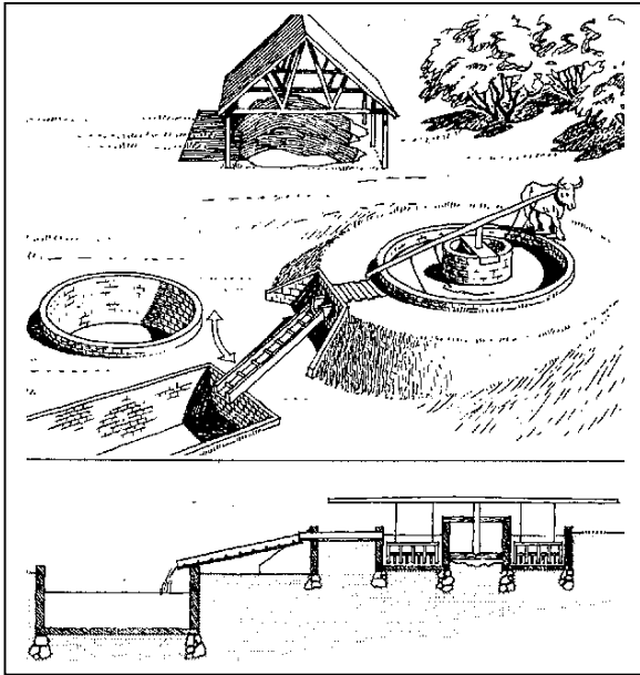
Fig. 1-7 Animal powered washmill for clay cleaning. A grooved tray leads to the settling tanks
