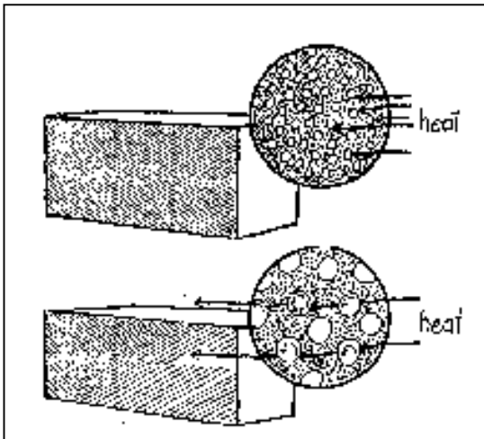
Fig.1-42: Heat going through a sawdust insulating brick is stopped by all the pockets of air left by the burned out sawdust particles.; Fig.1-43: If the insulating holes are too big the air inside the holes can rotate and thereby heat is transferred through the brick.
