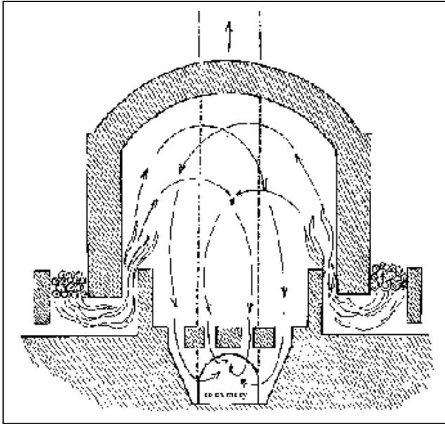
Fig.2-16: Down-draught kiln with flue channels under the floor
