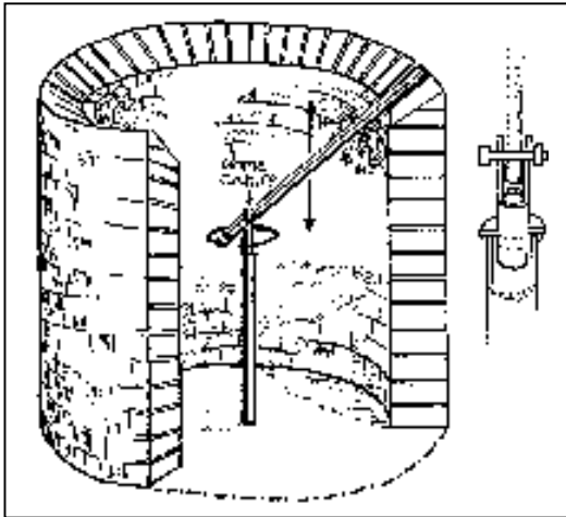
Fig.2-99: Arrangement of dome ruler.
