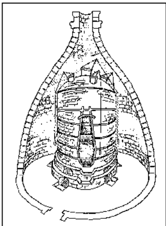
Fig.2-13: Cross-section of a hovel kiln
