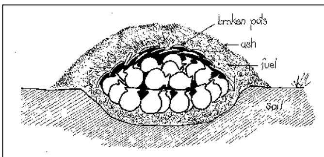
Fig.2-1: Bonfire kiln
