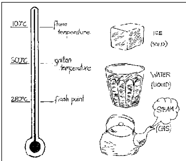
Fig.2-46: Temperatures of flash point, ignition and flame of wood; Fig.2-47: Water in its three forms.
