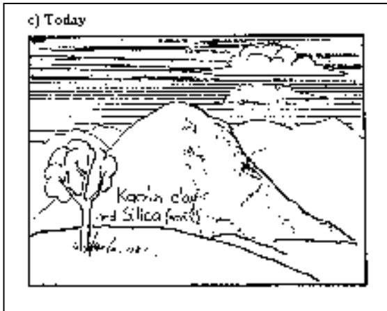
Fig. 1-2: Exposed to the action of weather the feldspar rock is slowly changed into clay. Chemically this change is written:
