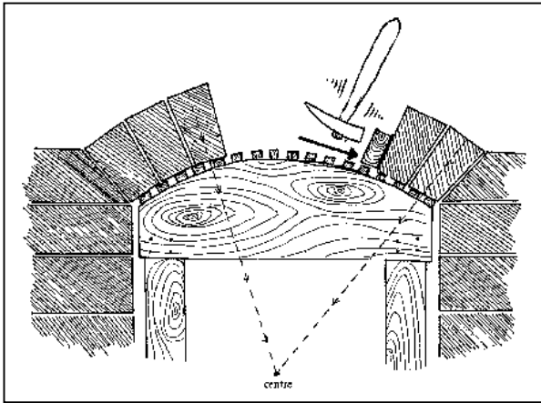
Fig.2-95: Laying the arch
