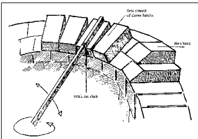
Fig.2-100: Skewbacks are laid as headers.
