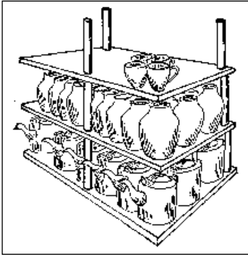
Fig.2-128: Slabs should be supported at three points only if possible.
